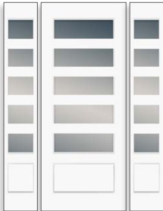
Door: 3/0 8/0 2664-010-C-1-SO3-5H Sidelites: 1/2 8/0 764-010-C-1-SO3-5H
