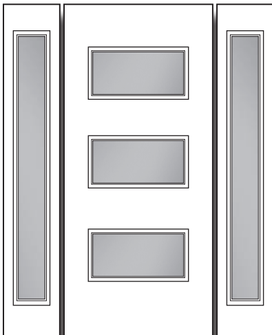
Door Glass Size: 22" x 10" (x3) • 22" x 15" SOL (x3) Sidelite Glass Sizes: 6'8": 7" x 64"
