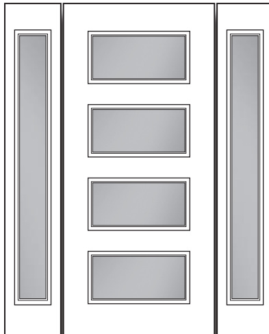
Door Glass Size: 22" x 10" (x4) • 22" x 15" SOL (x4) Sidelite Glass Sizes: 8'0": 8" x 80"
