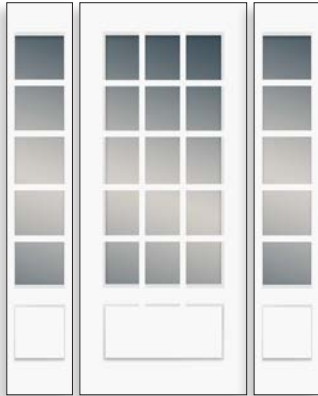
Door: 3/0 6/8 2648-010-C-1-SO-3W5H Sidelites: 1/2 6/8 848-010-C-1-SO-5H
