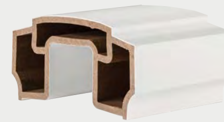
Top Rail Size: 5.4"W x 2.7"H
